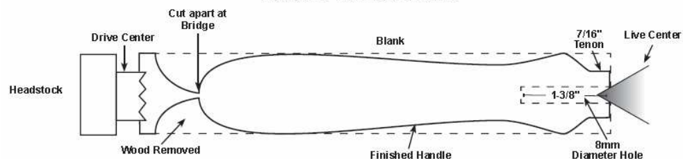
Diagram B - Turning the Handle
