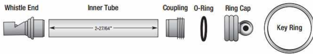
DIAGRAM A • Whistle/Key Ring PARTS
